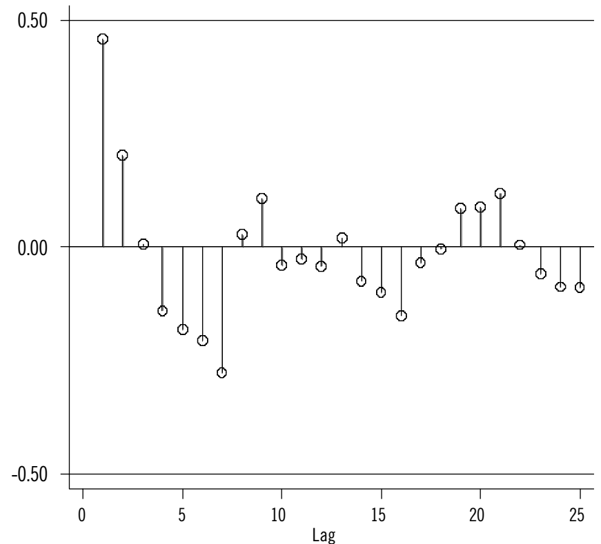
Figure 1 – Autocorrelation Function Plot of the Attacks Series
